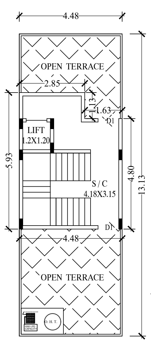
PROPOSED TERRACE FLOOR PLAN
